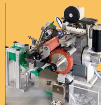
"HSC-Kompakt" automation "Rotary" tampon printing
