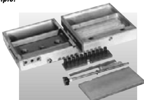
from top to bottom: cliché holder (left), ink well (right), doctor blade carrier, ink spatula, ink spatula holder, steel cliché
